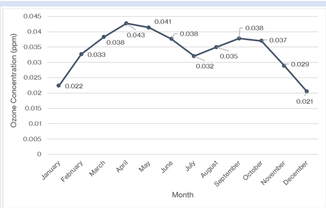
Figure 14: Average Monthly Max Ozone Concentration at Los Angeles and Long Beach Port 2010-2019 (EPA Sensor: 60374006)
