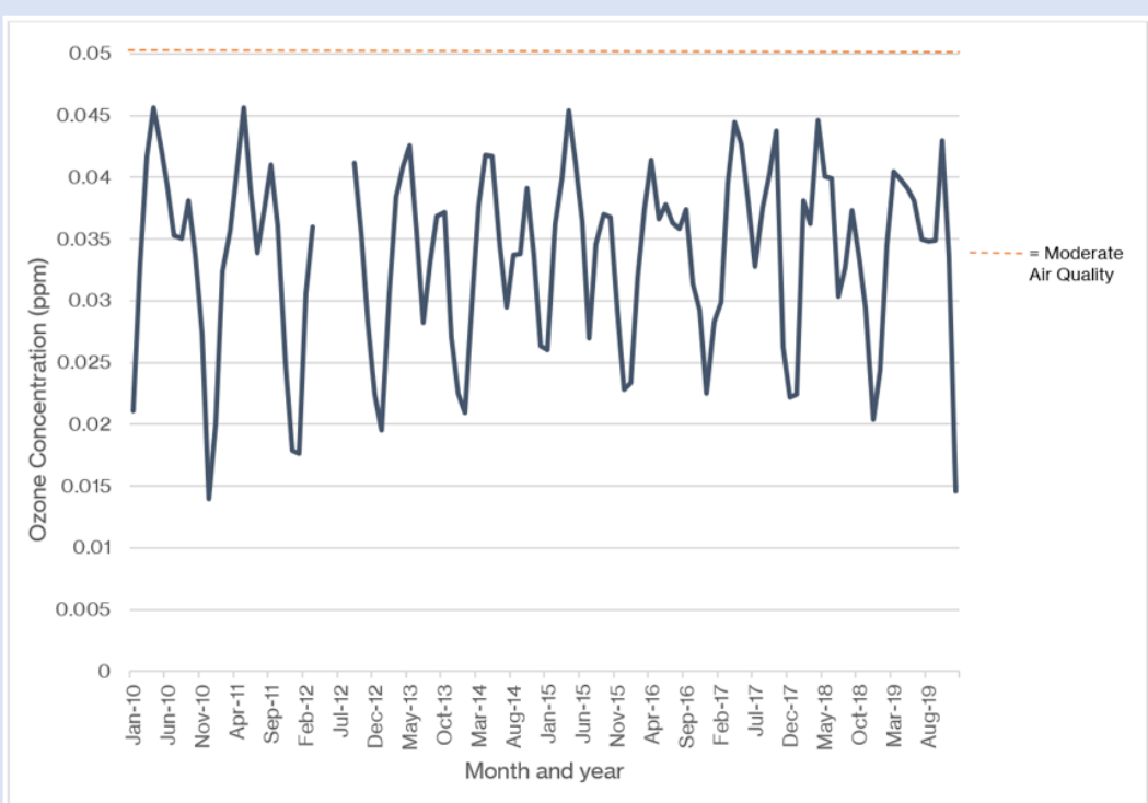
Figure 13: Ozone Concentration at Los Angeles and Long Beach Port 2010-2019 (EPA Sensor: 60374006)
