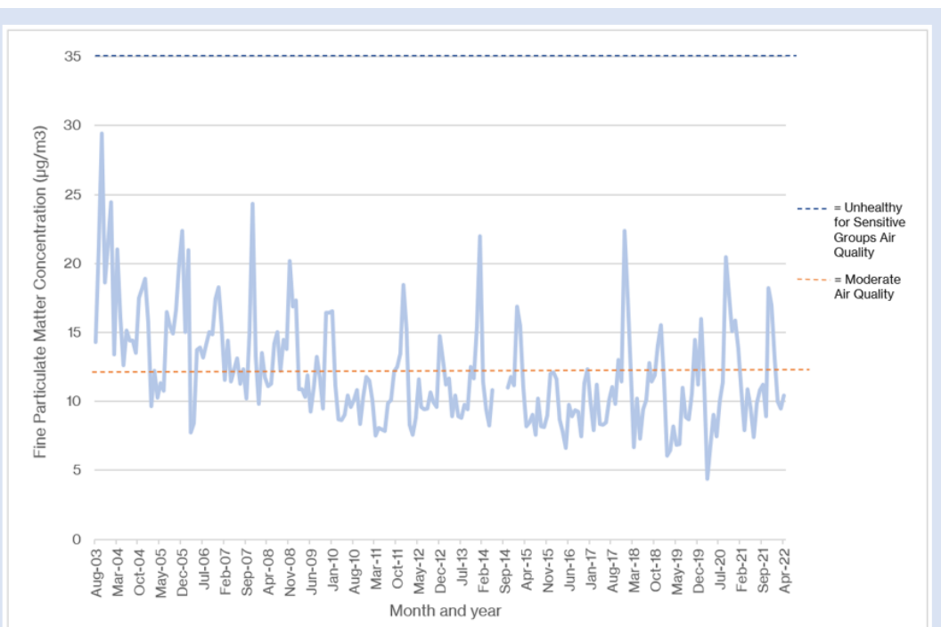
Figure 11: Fine Particulate Matter Concentration at Los Angeles and Long Beach Port 2003-2022 (EPA Sensor: 60374004)
