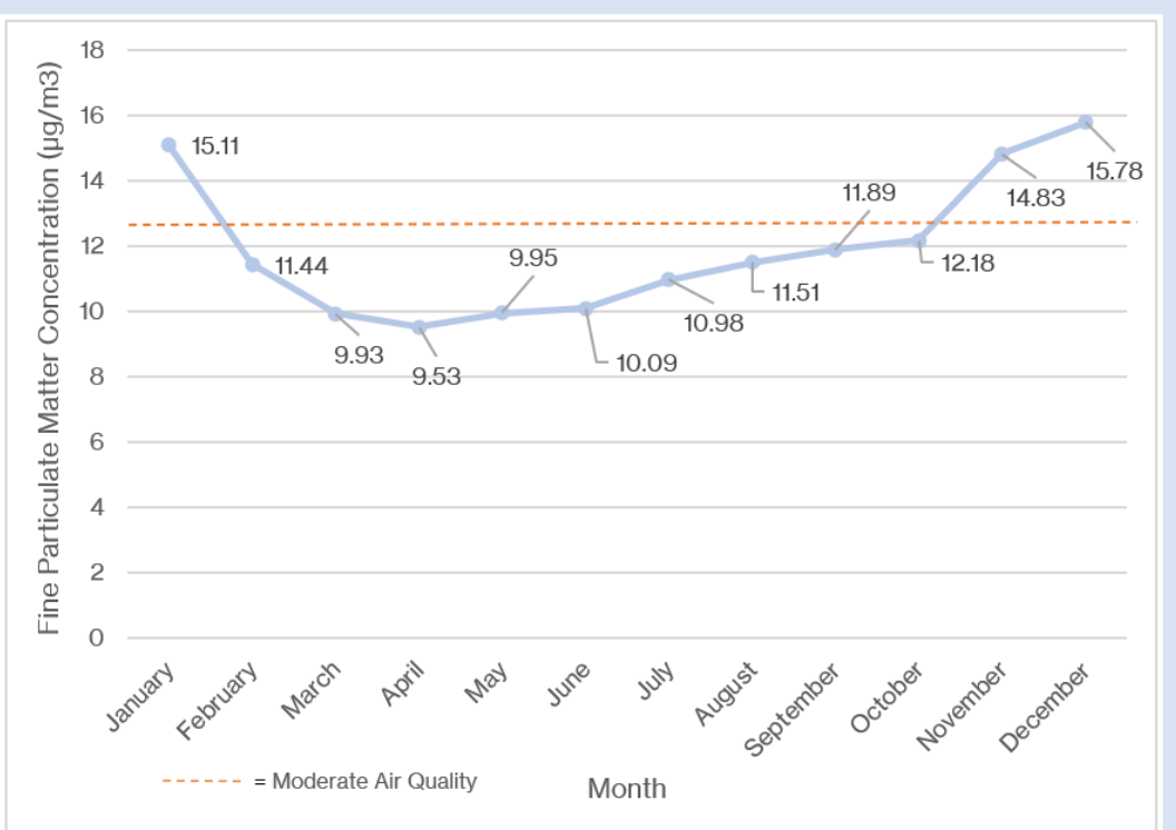
Figure 12: Average Monthly Fine Particulate Matter Concentration at Los Angeles and Long Beach Port 2003-2022 (EPA Sensor: 60374004)
