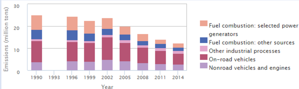
Figure 8: Anthropogenic NO x emissions by source category in the U.S. 1990 – 2014 (Source: U.S. EPA)
